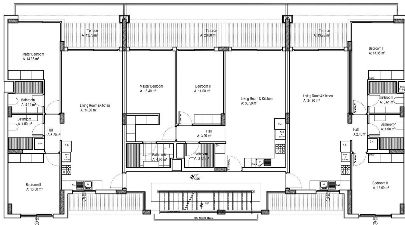
FIRST FLOOR
