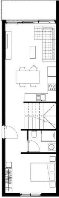
FIRST FLOOR
