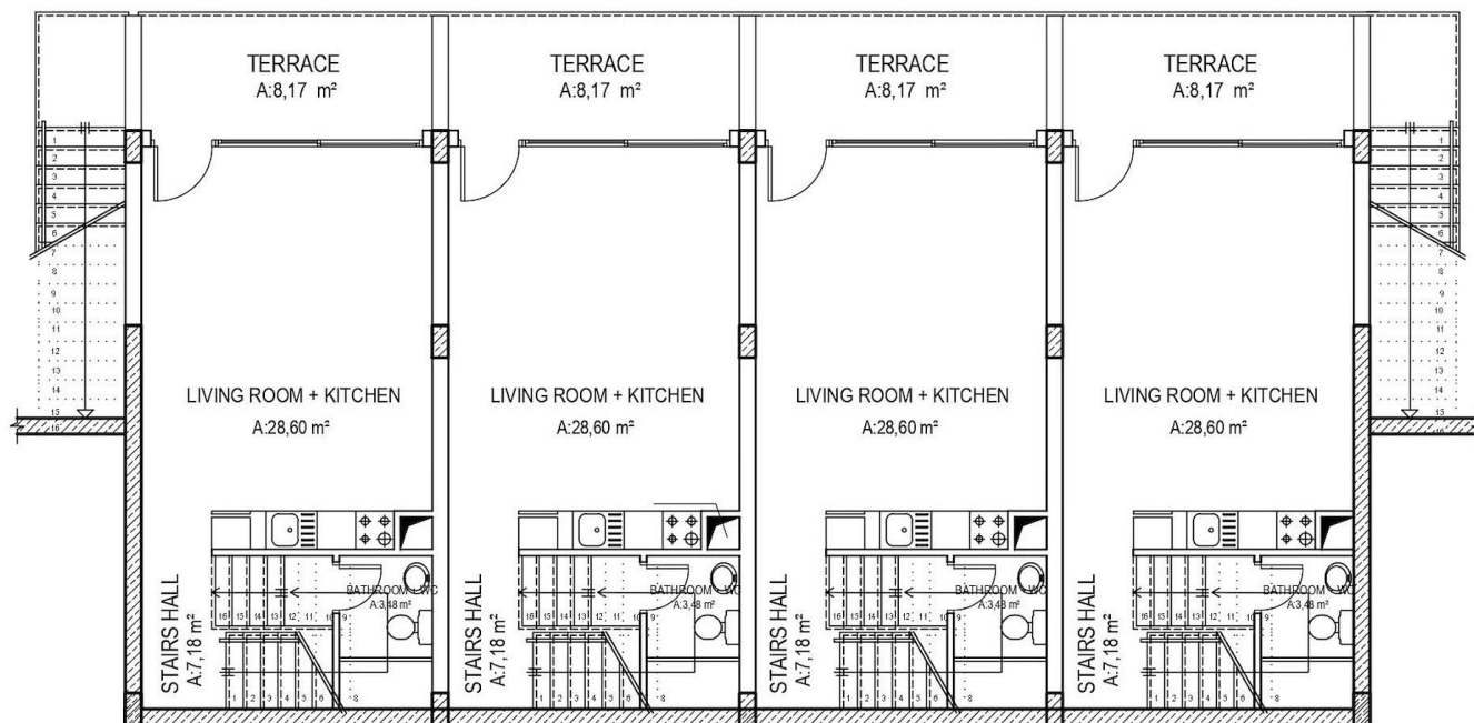
FLOOR PLAN
