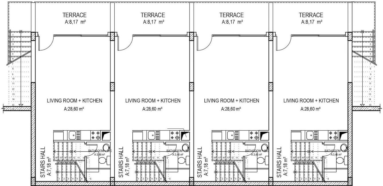
FLOOR PLAN
