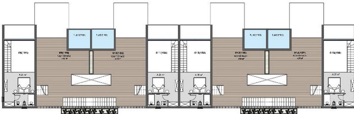
MEZZANINE PLAN
