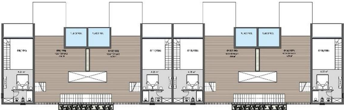
MEZZANINE PLAN
