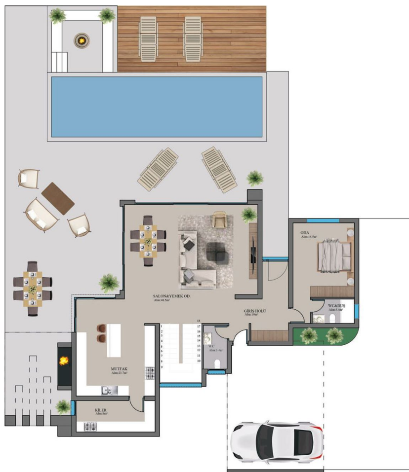
TİP A ZEMİN KAT PLANI BRÜT ALAN:191.5M2+42M2 OTOPARK ALANI
