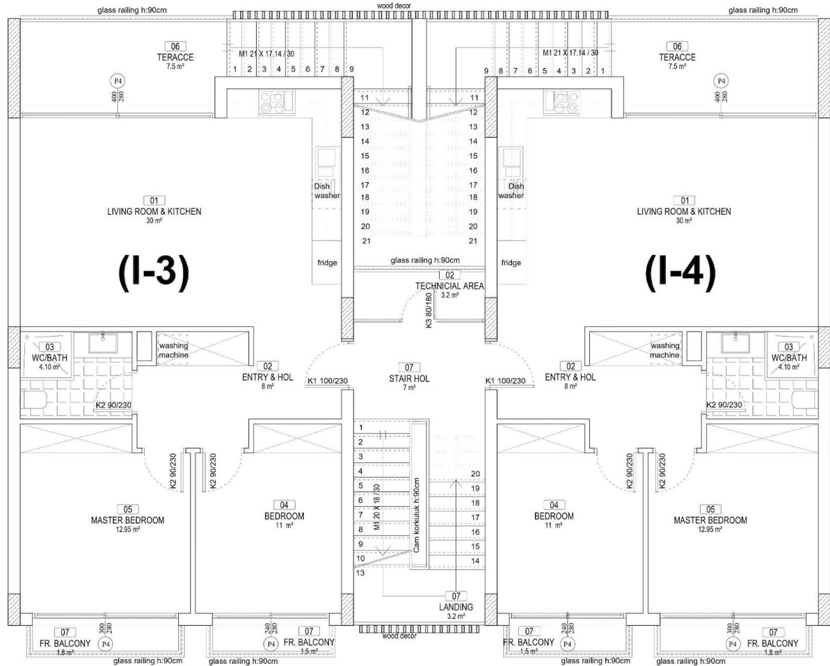
TYPE I FIRST FLOOR PLAN(2+1)
